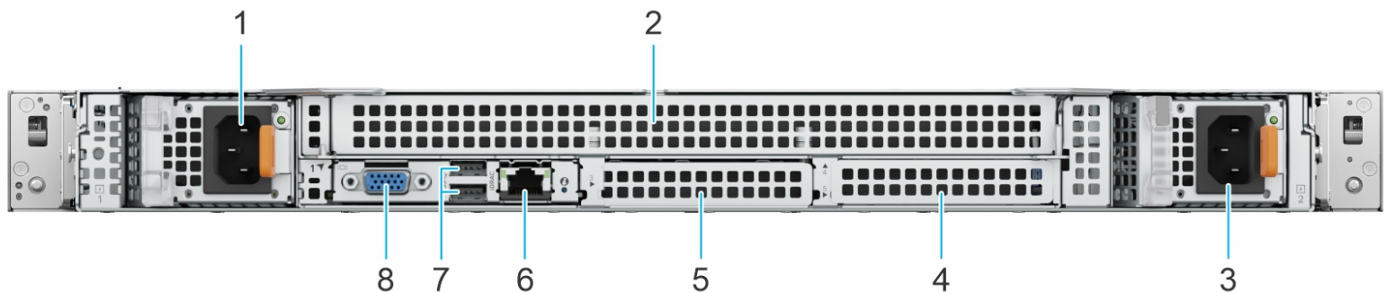
Figure 9. Rear view of the system with 8 x EDSFF E3.S drive system with front I/O
