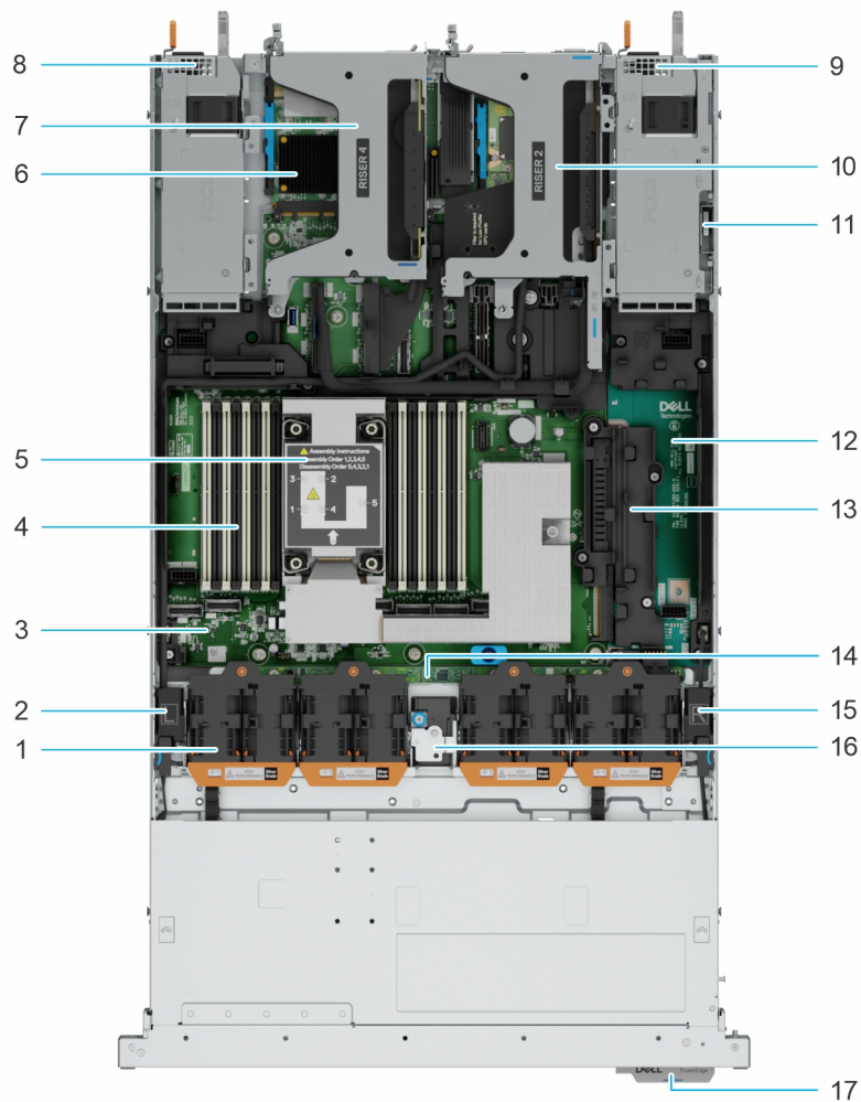
Figure 12. Inside the system with rear I/O configuration
