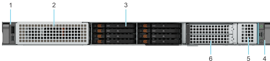
Figure 3. Front view of 8 x EDSFF E3.S -drive system with rear I/O
