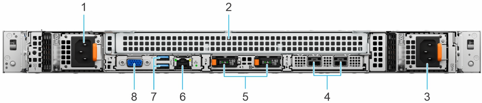
Figure 8. Rear view of the system with 8 x 2.5 inch drive system
