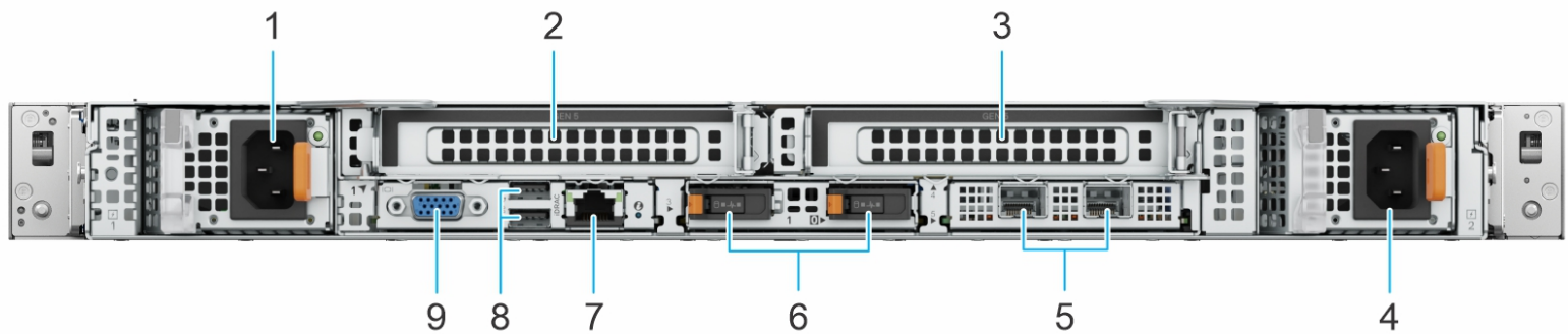
Figure 10. Rear view of the system with 8 x EDSFF E3.S drive system with rear I/O
