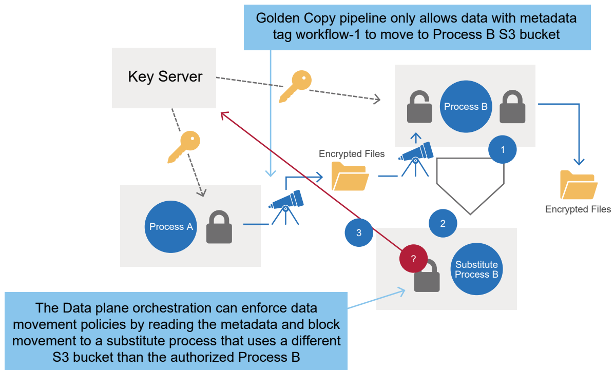
Diagram 1 Golden Copy Metadata Data Movement Policy Enforcement
