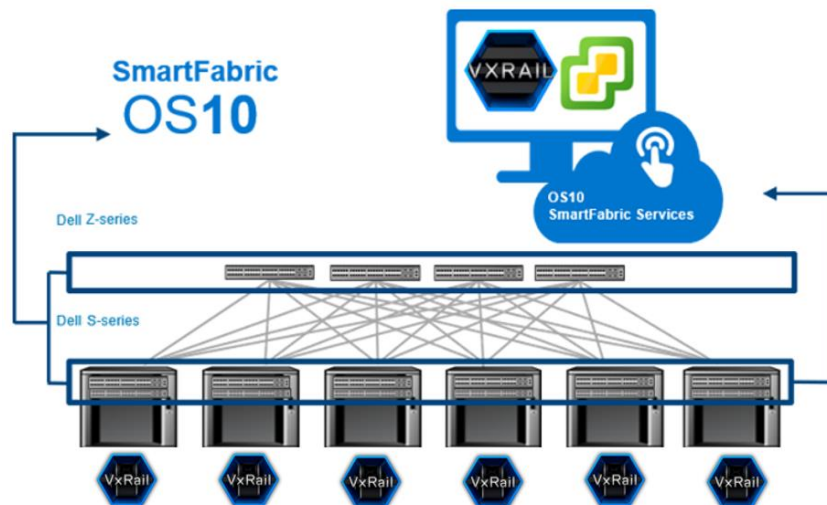
Figure 22. VxRail with SmartFabric Services
