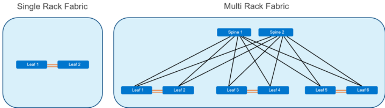
Figure 23. SmartFabric enabled multi-rack network expansion
